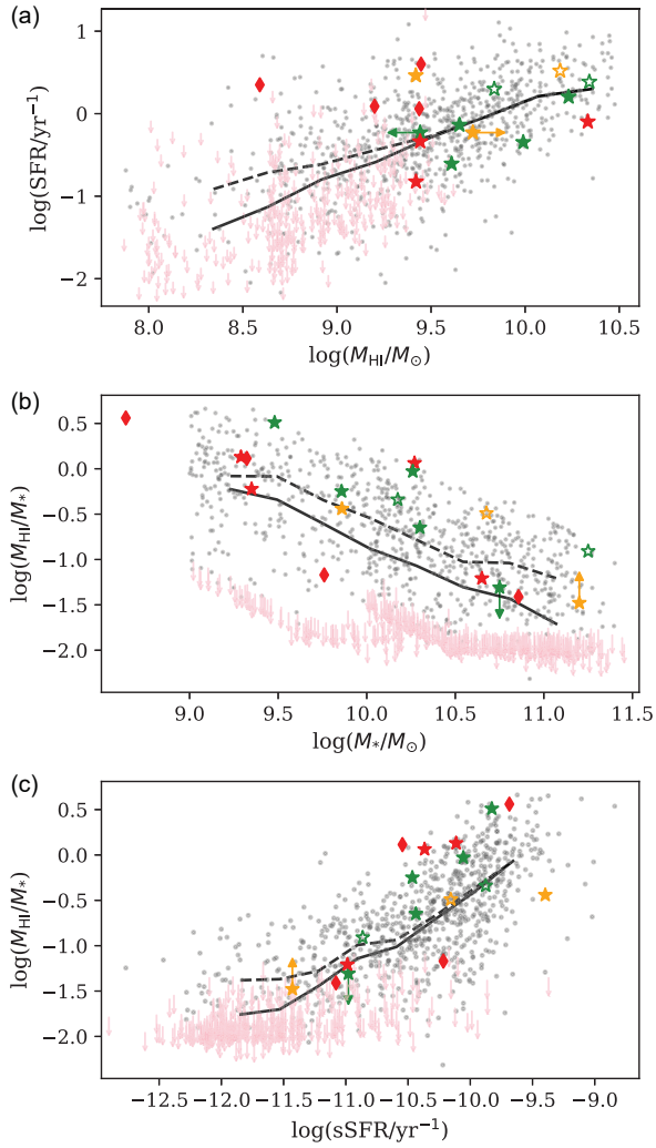
Figure D1. Same as Figure 8 but with targets coloured by disturbance classification.
