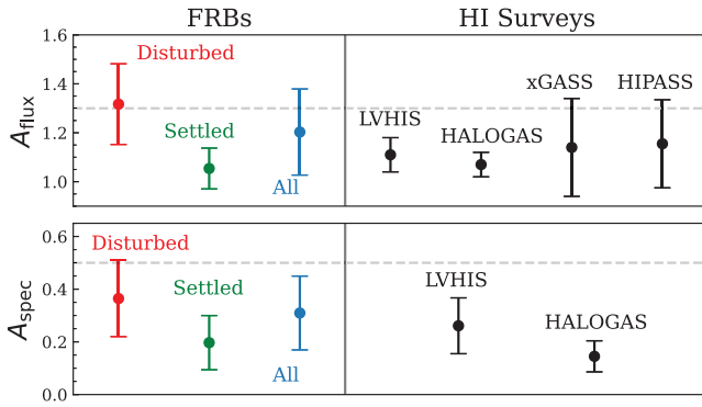
Figure 7. A_{flux} and A_{spec} values of FRB hosts compared to background populations presented in Reynolds et al. (2020b), Watts et al. (2020). LVHIS and HALOGAS sample low-density environments, whereas xGASS is more representative of the local galaxy population. The xGASS result is an approximation; we generate the results by extracting the cumulative distribution of Fig. 2 from Watts et al. (2020). The two dashed lines indicate our chosen thresholds for asymmetry, outlined in Section 4.2.
