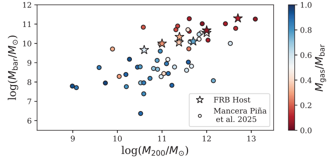
Figure 9. Baryonic vs. virial masses for FRB hosts and the sample of Mancera Piña et al. (2025).
