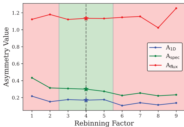
Figure B1. 1D asymmetry metrics for FRB 20210405I at various resolutions.
