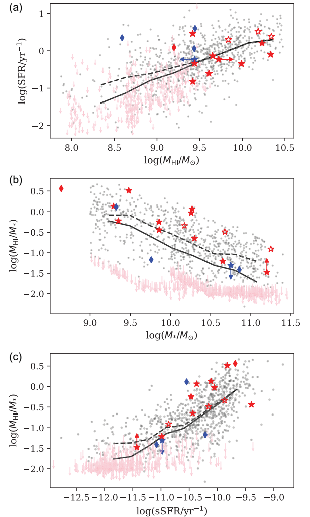
Figure 8. Global HI properties of FRB hosts, separated into non-repeating (red) and repeating (blue) FRBs. Stars indicate our sample, and diamonds indicate the previously published hosts. These are overlaid on the xGASS sample (grey = detected in HI, pink = non-detections in HI) (Catinella et al. 2018). The FRB host stellar masses and SFRs are taken from literature SED modelling values where possible; open stars represent hosts without SED fitting, where we derive M_* from literature K -band luminosities and use our radio continuum SFR estimates (see Table 3). The black lines indicate the median values at eight arbitrary bins along the x-axis for all xGASS galaxies (solid line) and for just HI detected galaxies (dashed line).
