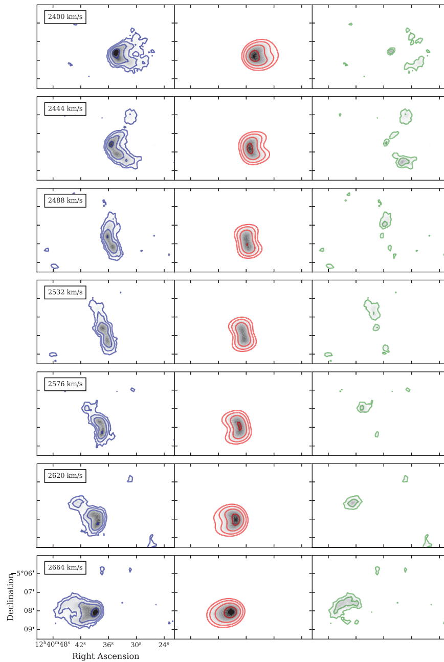
Figure C1. Comparison between observations of the host of FRB 20200723B (left) and a smooth rotating disk model from 3DBarolo (centre), with residuals shown (right).
